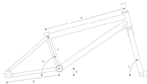
FRAME GEOMETRY
