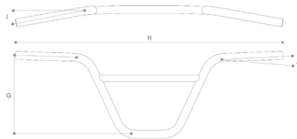
BAR GEOMETRY
