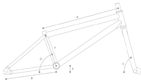
FRAME GEOMETRY
