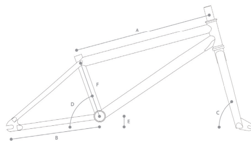
FRAME GEOMETRY
