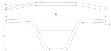
BAR GEOMETRY
