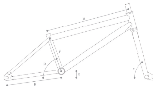
FRAME GEOMETRY
